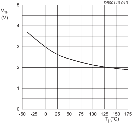
V_{DS} = V_{GS}; I_{DS} = 20\text{ mA} Fig. 13. Threshold voltage as a function of junction temperature
